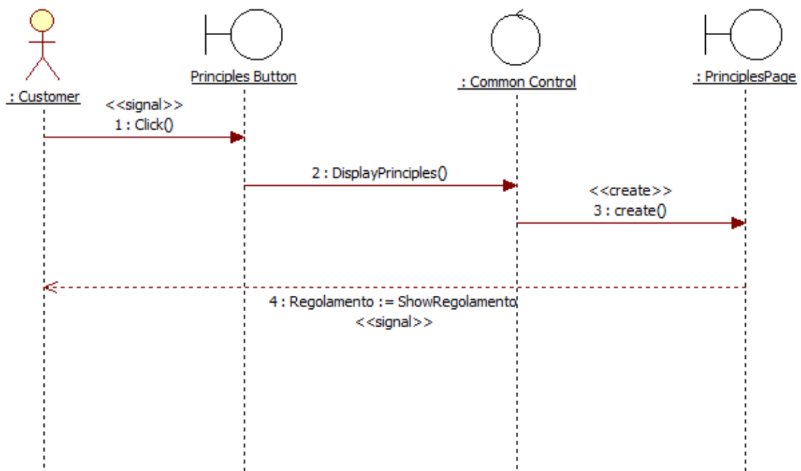
Figura 22 - Sequence Diagram SD04 Display principles
