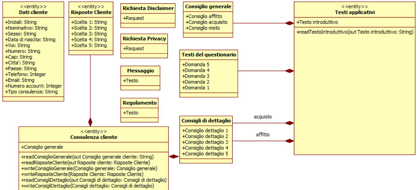
Figura 17 - Class Diagram: Domain Classes
