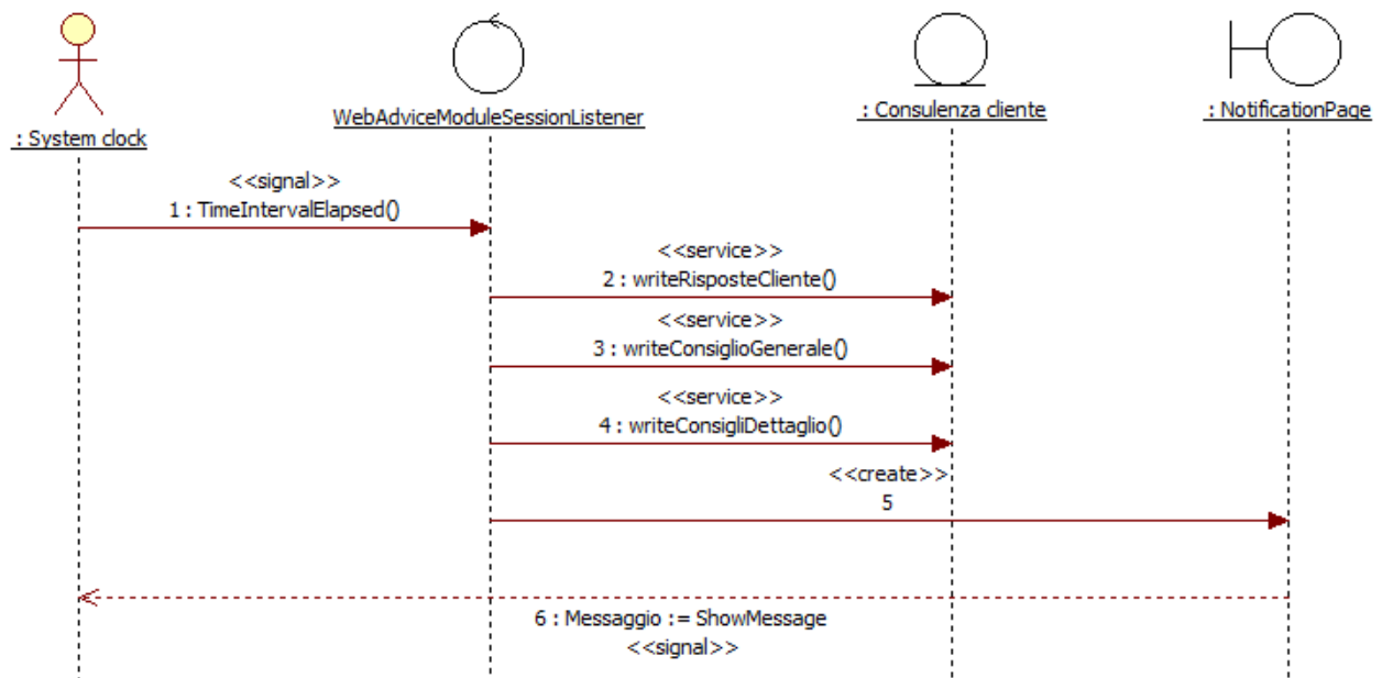
Figura 25 - Sequence Diagram SD08 Display time-out
