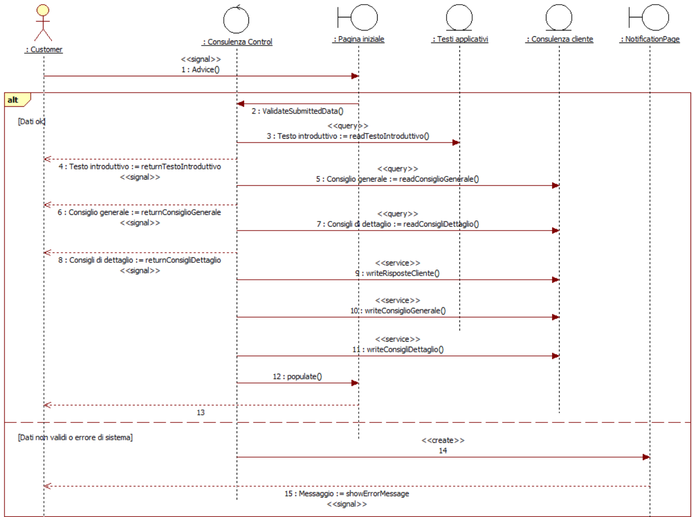
Figura 18 - Sequence diagram SD01 Display rent or buy advice
