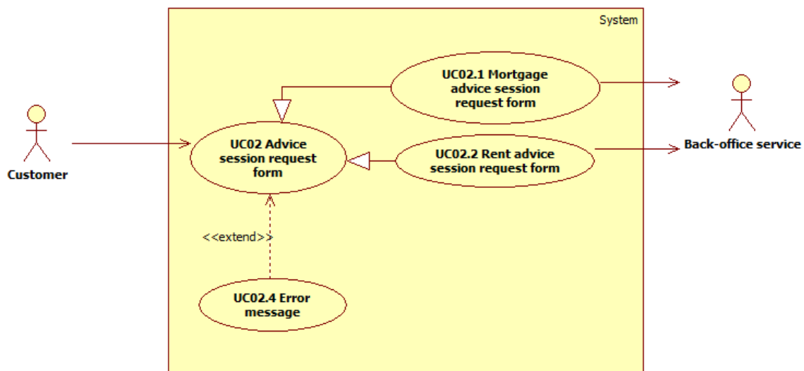
Figura 11 - Use case Advice session request form
