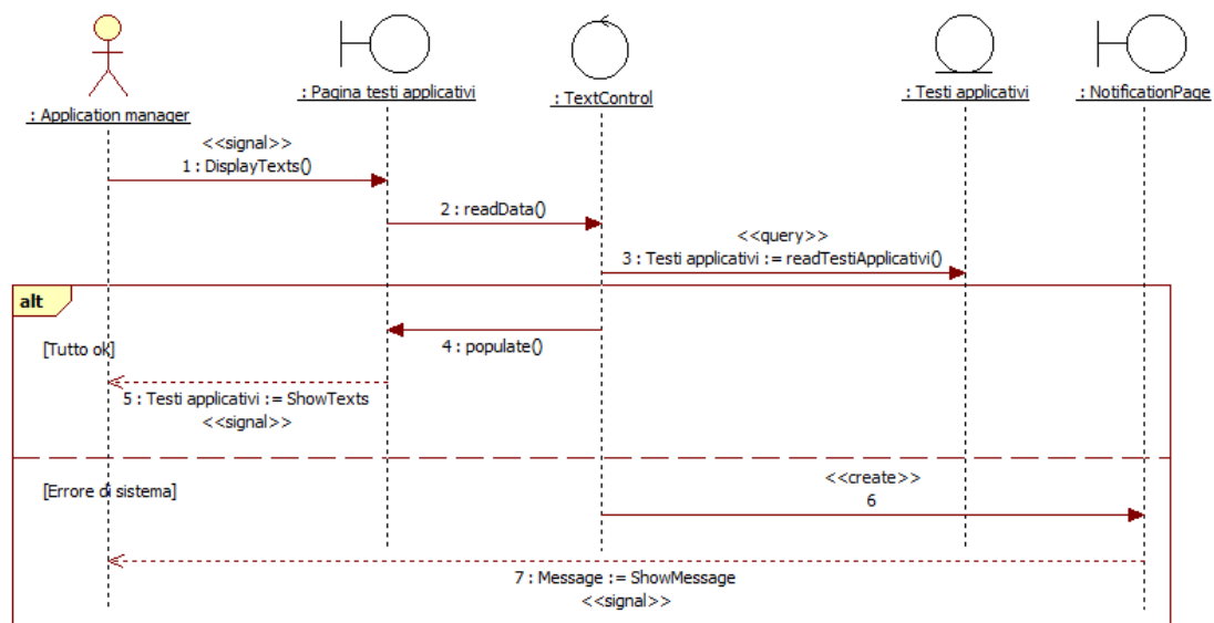
Figura 20 - Sequence Diagram SD03 Select Text
