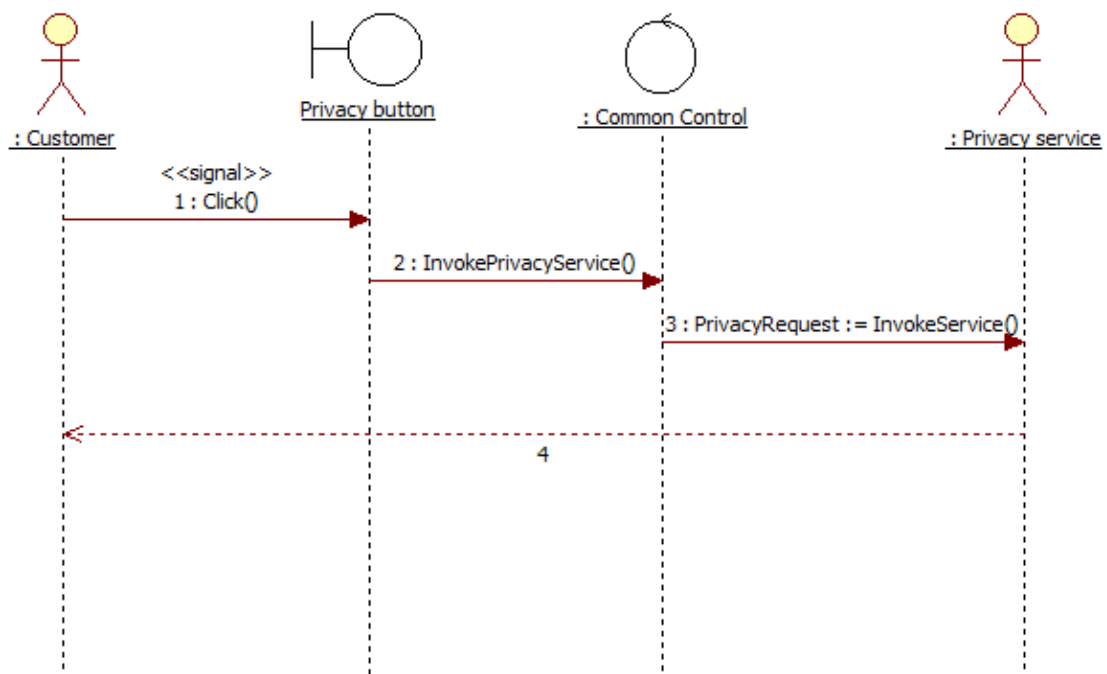
Figura 24 - Sequence Diagram SD07 Invoke Privacy Service
