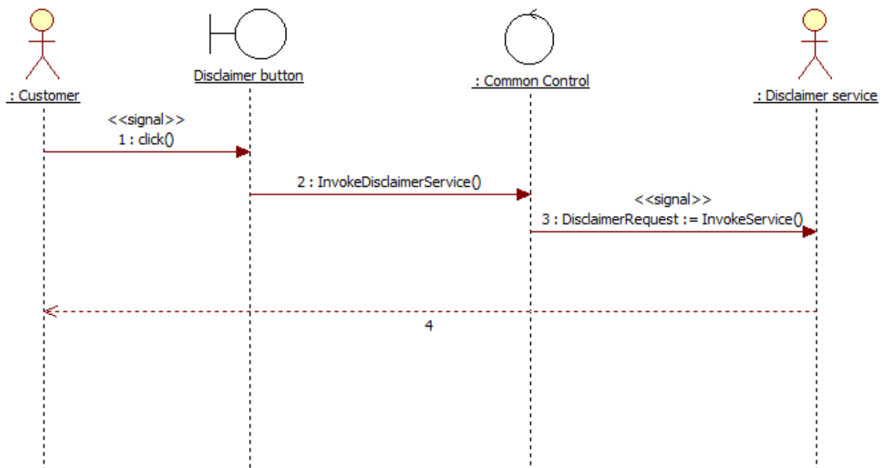
Figura 23 - Sequence Diagram SD06 Invoke Disclaimer Service
