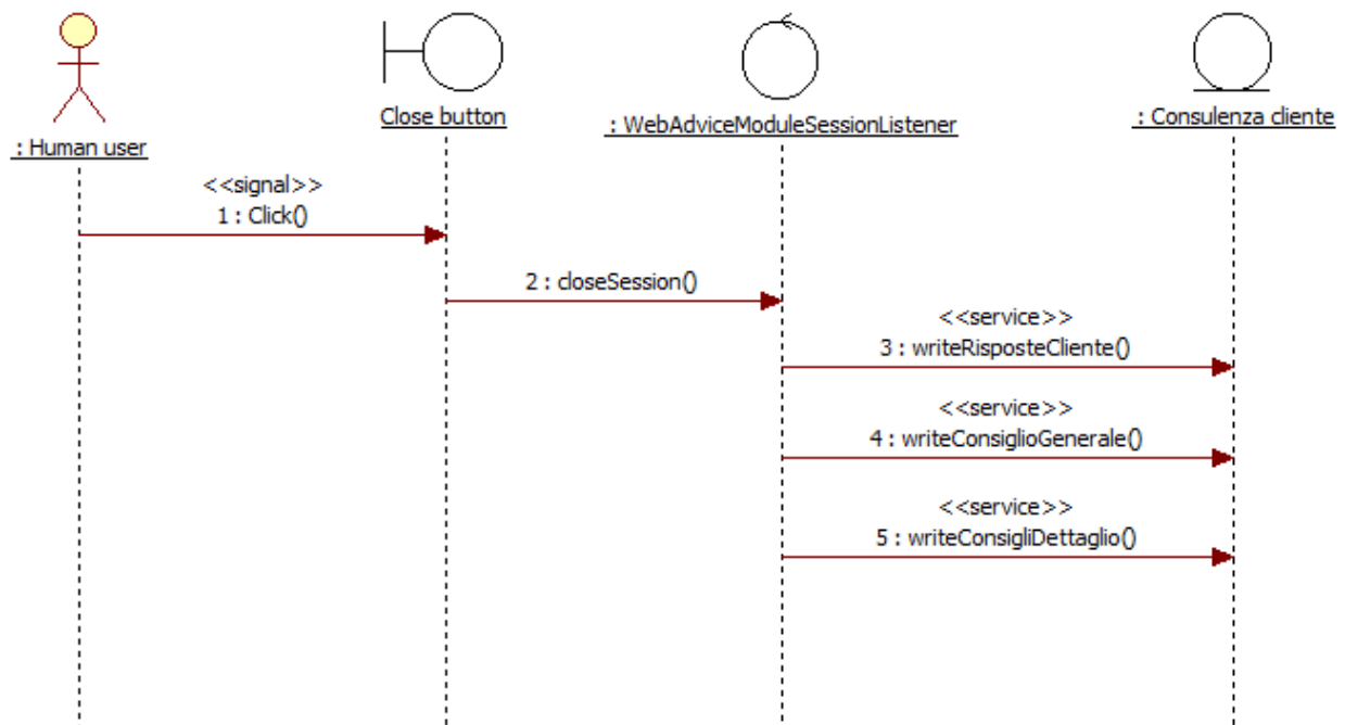
Figura 26 - Sequence Diagram SD09 Close module
