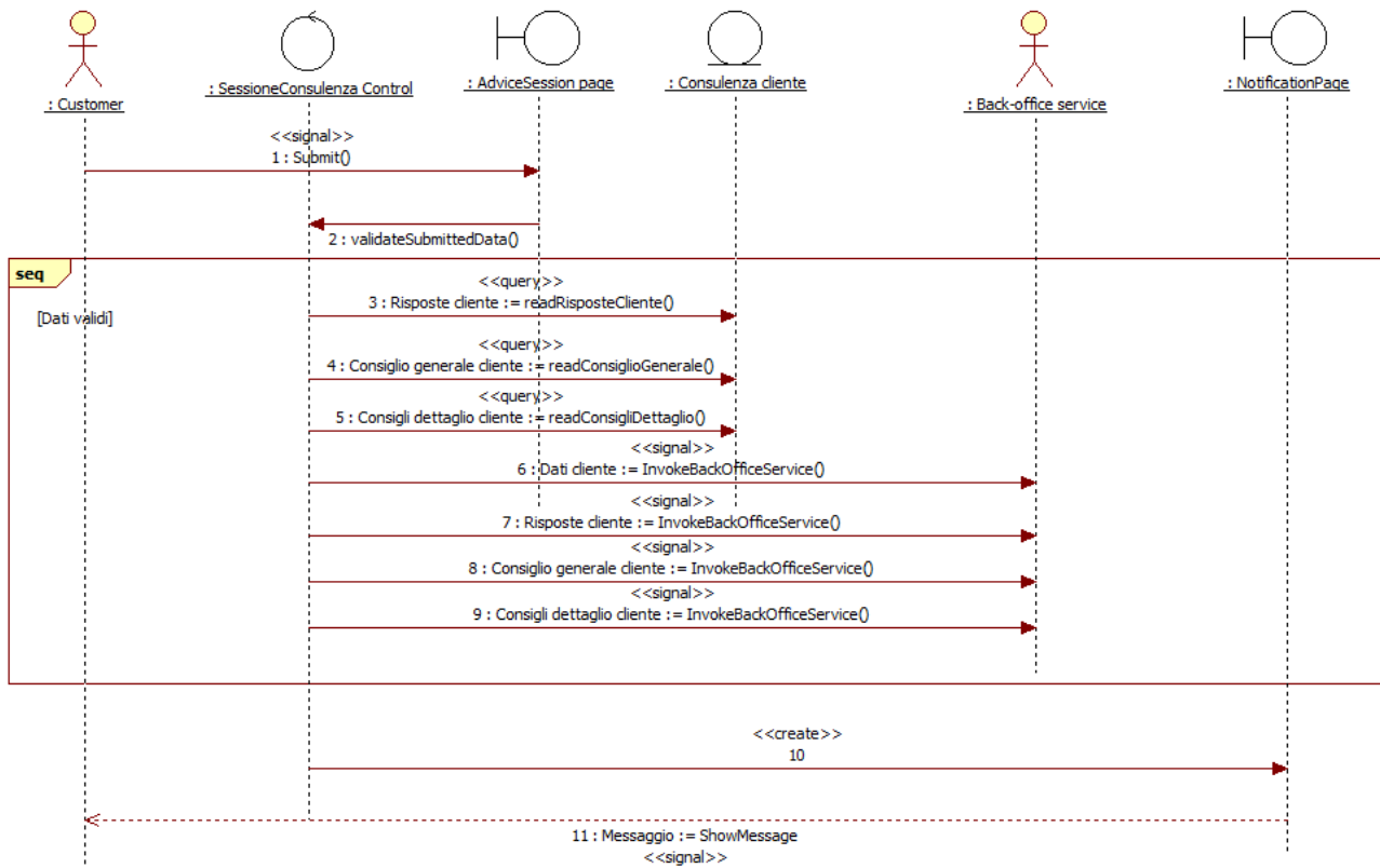
Figura 19 - Sequence Diagram SD02 Advice session request form
