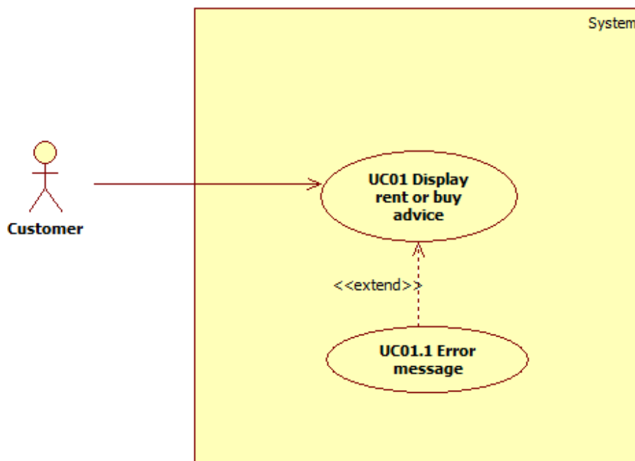
Figura 10 - Use case Display rent or buy advice
