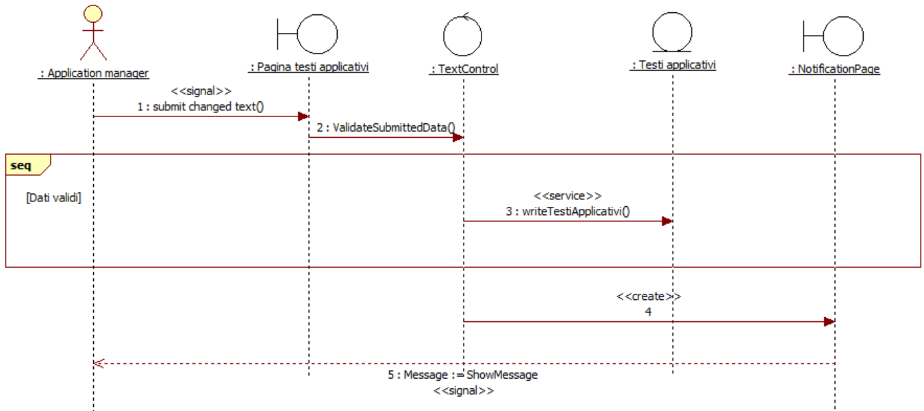
Figura 21 - Sequence Diagram SD04 Edit Text
